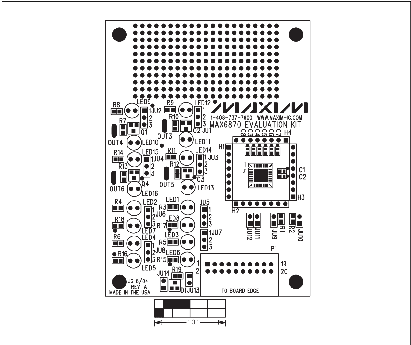
Figure 10. MAX6870 EV Kit Component Placement Guide—Component Side
